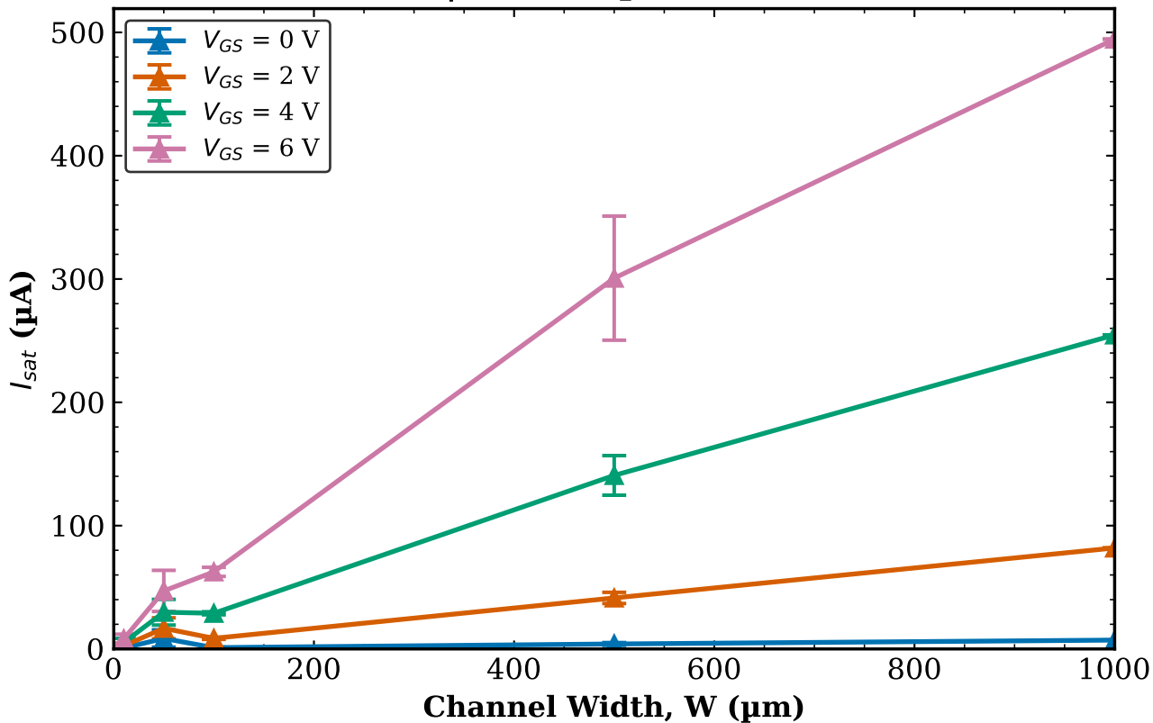
All Chips - Combined I_{sat} vs W | L = 20\text{ }\mu\text{m} (mean \pm std)
